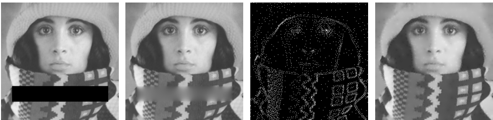
(a) Arbitrary data (b) Reconstruction (c) Optimal data (d) Reconstruction Figure 2. (a) Image data with an arbitrary missing rectangular region (marked in black). (b) Corresponding reconstruction with (1.1). The reconstruction suffers from blurring effects. (c) Remaining data (5% of all pixels) with optimal reconstruction property. Missing data is black. (d) Corresponding reconstruction with (1.1). The reconstruction is sharp although the Laplacian causes strong smoothing. Source original image: [49]
