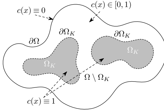
Figure 3. Visualization of the setup specified in (2.4) with a nonbinary valued mask function c .
